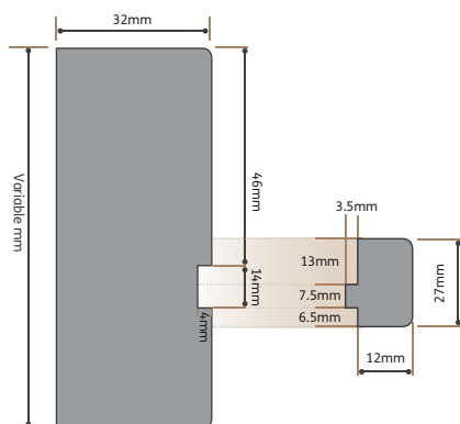
Standard lining components
