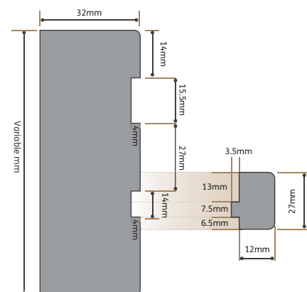
Fire Door lining components
